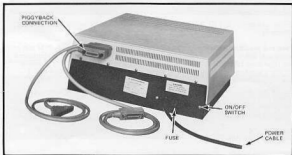
Figure 10 — Model 2040 Dual Drive Floppy Disk, Rear View
