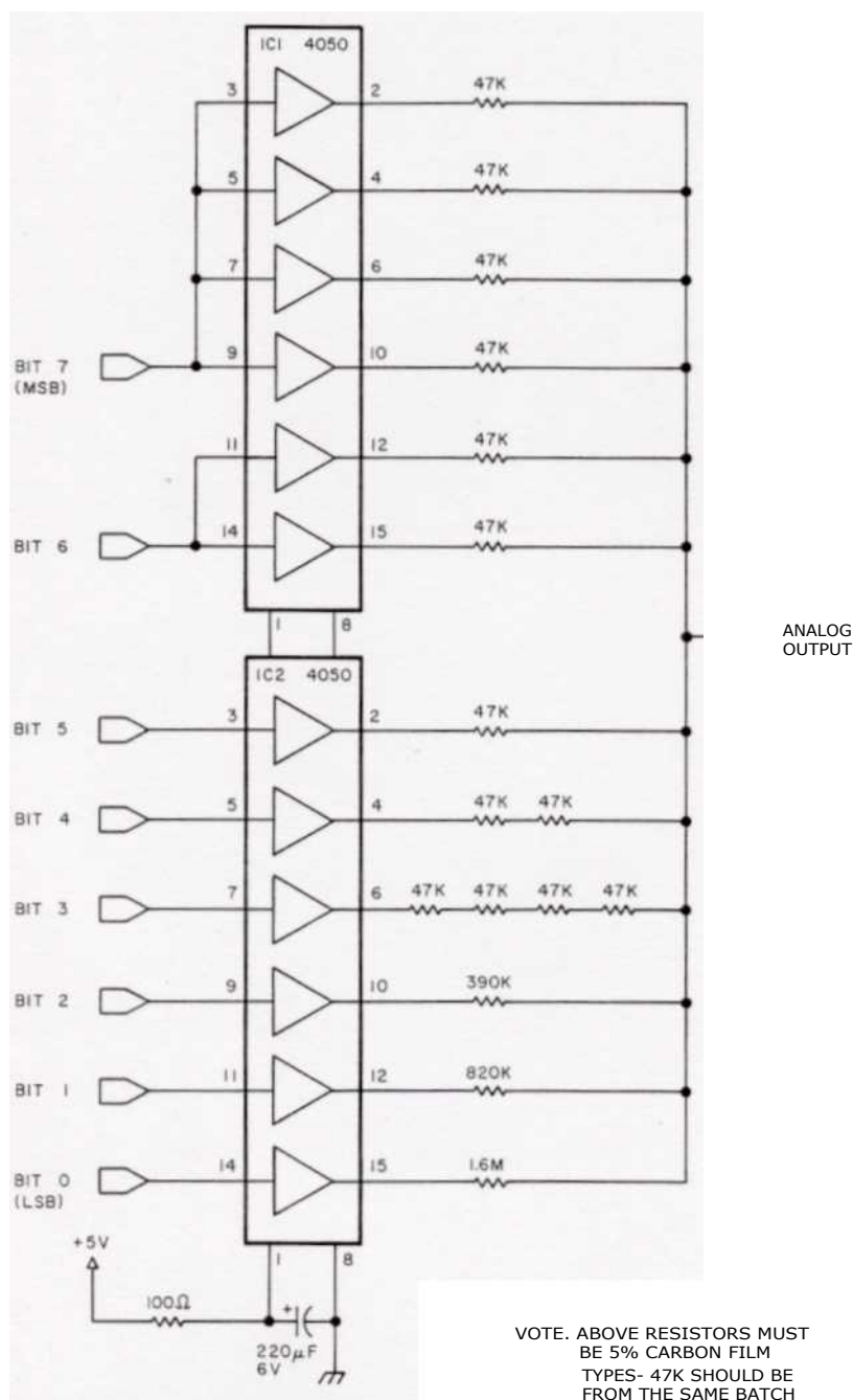
Figure 3: An 8 bit digital to analog converter (DA C). This circuit accepts an 8 bit binary number from the output port and generates a corresponding DC voltage as its output. The output voltage from this circuit is equal to ((I/255) \times 5) V, where I is the decimal equivalent of the 8 bit input which can take on any value from 0 to 255.
