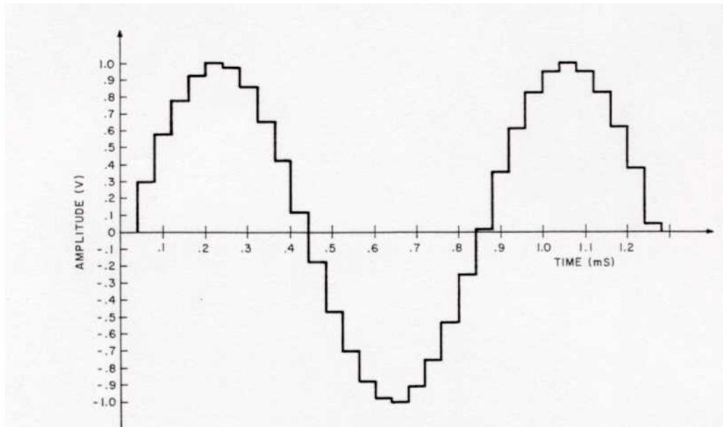
Figure 4: A sine wave as it would appear at the output from the digital to analog converter shown in figure 3. Each step in the approximation of this wave is called a sample. This particular illustration shows a 1.2 kHz sine wave sampled at a rate of 25,000 samples per second. The resulting waveform is only a very rough approximation of the original, but low pass filtering can improve accuracy (see figure 5 and text).
