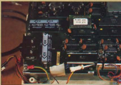
Flash installed in 1541 disk drive.
