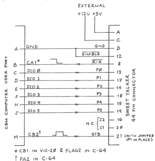
FIGURE 1. CBM/SWEET TALKER INTERFACE
